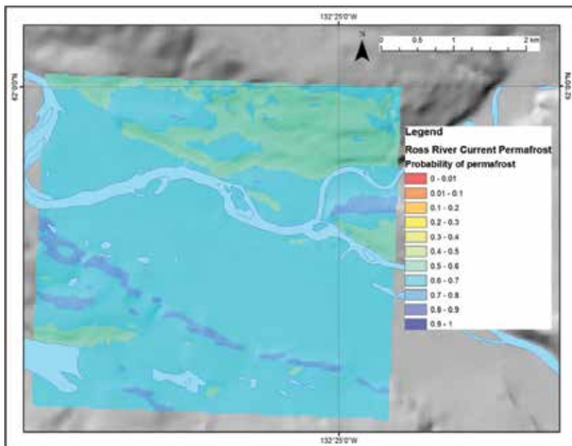
Figure 2.6.3.1 Permafrost probability under current climate conditions for the Ross River study area
