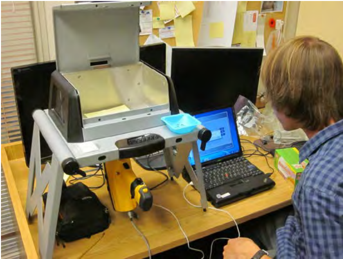
Figure 51 - Gavin operating XRF.
