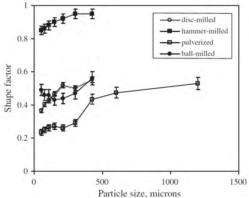
Figure 12 - Shape factor vs. particle size for gold grains in each grinding environment. Pulverizer produces the flattest grains across all sizes (Ofori-Sarpong & Amankwah, 2011).
